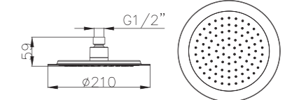
RS1023 Function: Spray φ 210mm
