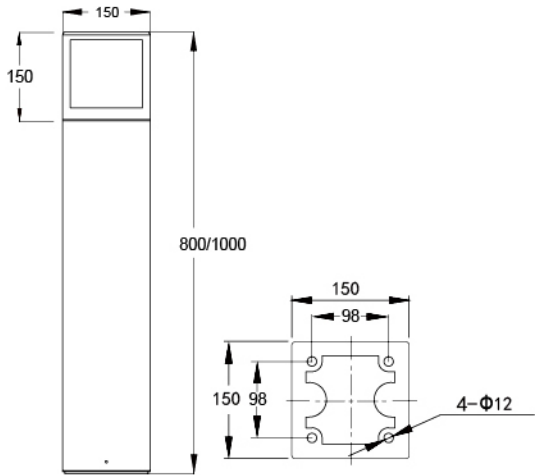
灯具尺寸 Product Dimensions(mm)
