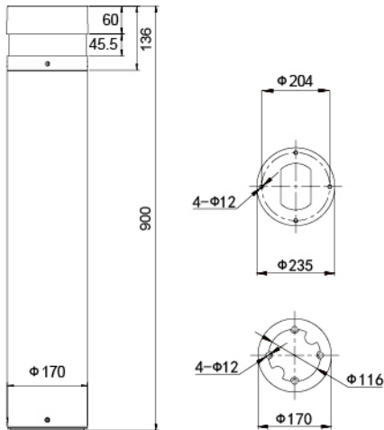
灯具尺寸 Product Dimensions(mm)
