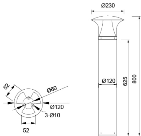
灯具尺寸 Product Dimensions(mm)
