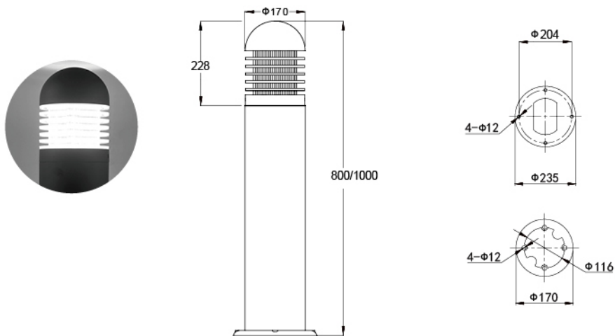
灯具尺寸 Product Dimensions(mm)
