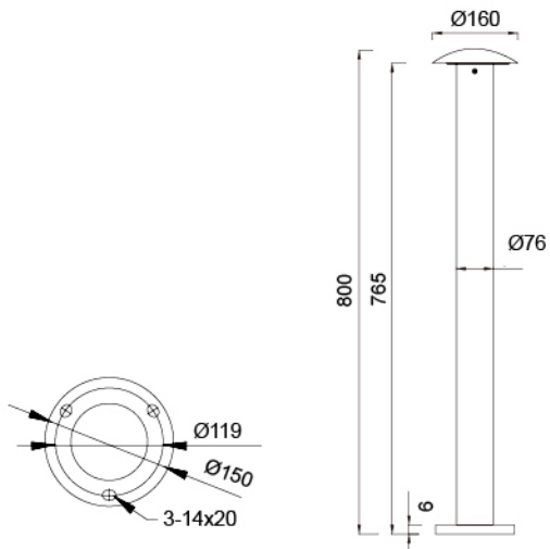
灯具尺寸 Product Dimensions(mm)
