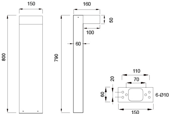
灯具尺寸 Product Dimensions(mm)
