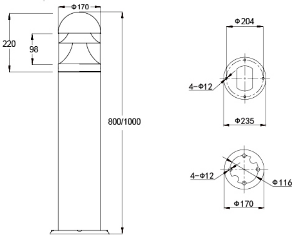
灯具尺寸 Product Dimensions(mm)
