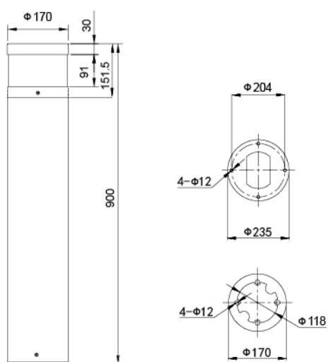
灯具尺寸 Product Dimensions(mm)
