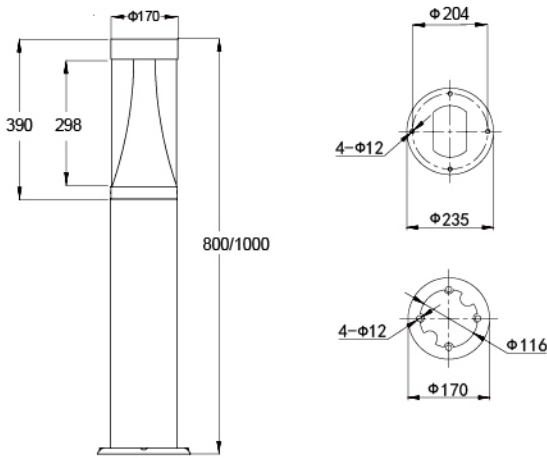
灯具尺寸 Product Dimensions(mm)
