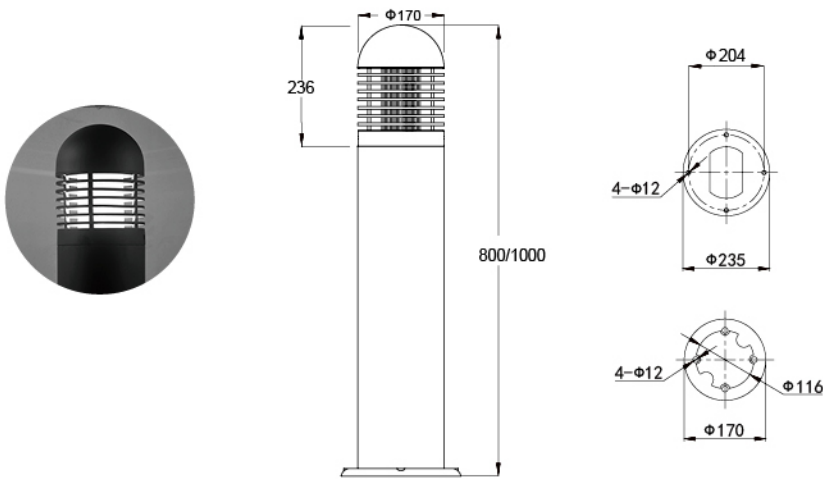
灯具尺寸 Product Dimensions(mm)
