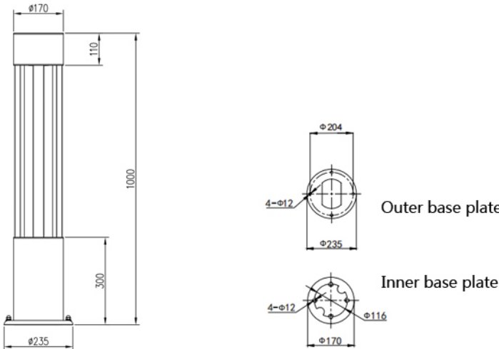
灯具尺寸 Product Dimensions(mm)
