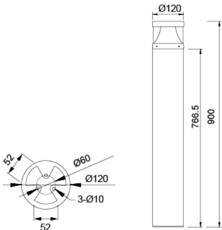
灯具尺寸 Product Dimensions(mm)
