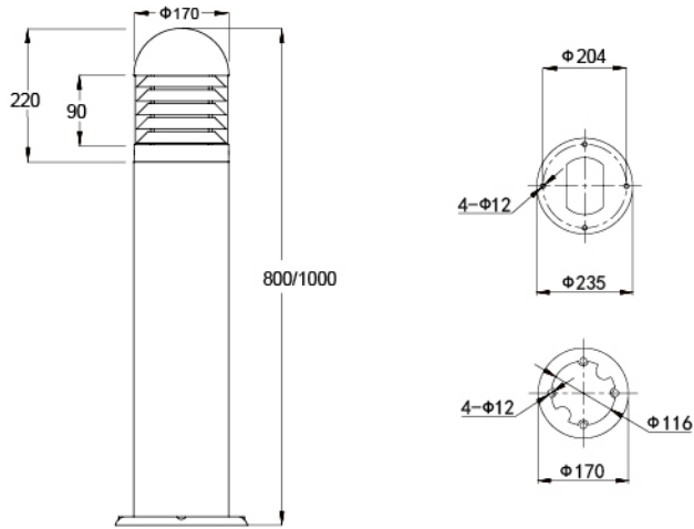
灯具尺寸 Product Dimensions(mm)
