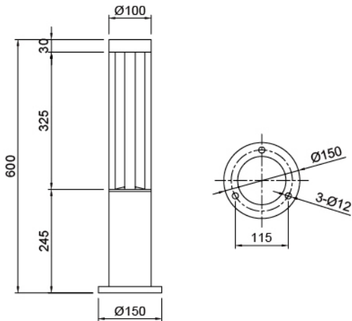
灯具尺寸 Product Dimensions(mm)
