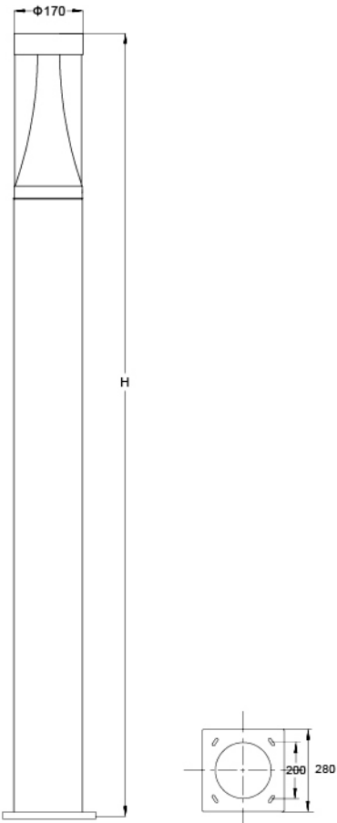
灯具尺寸 Product Dimensions(mm)
