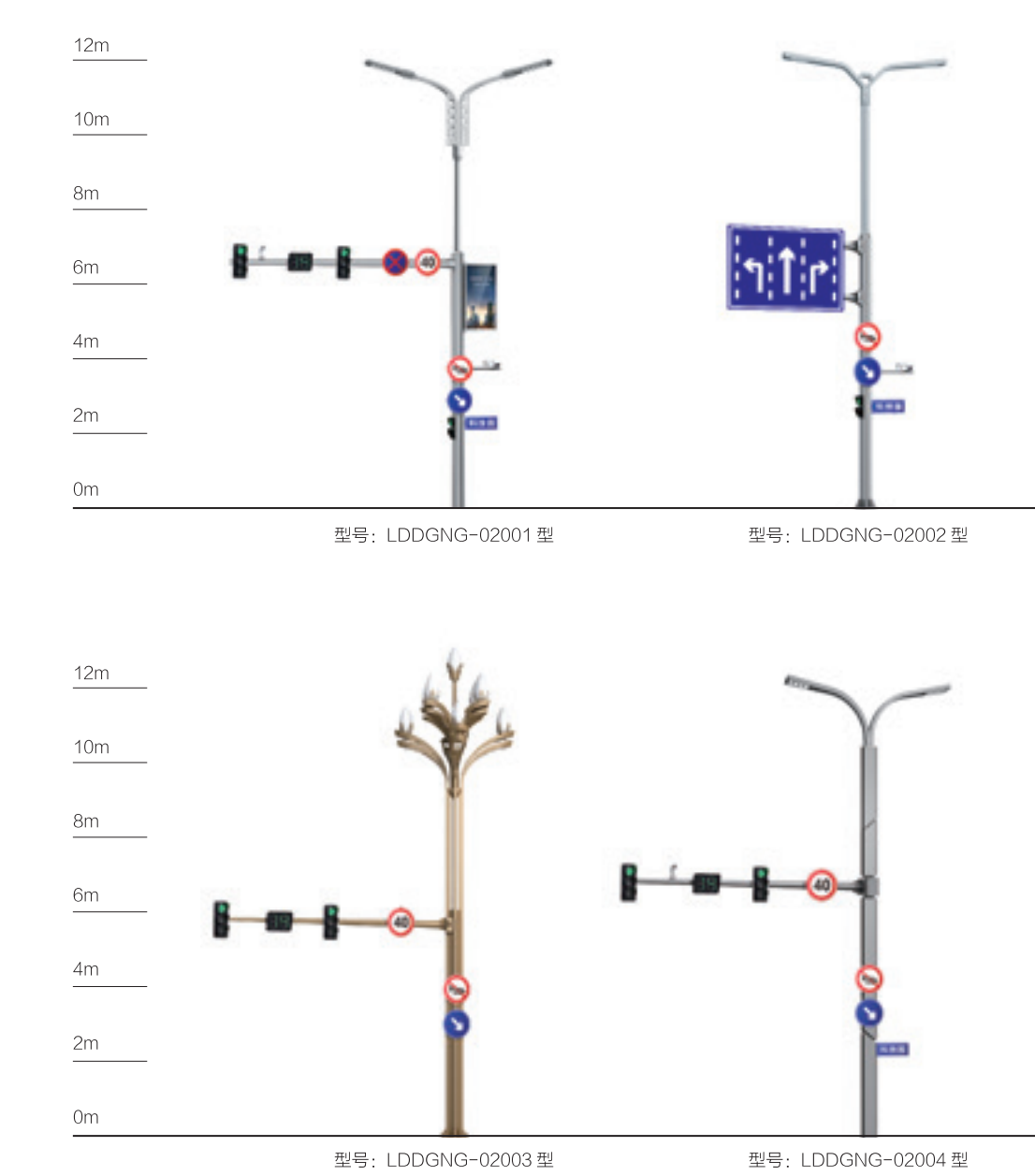
多功能智慧灯杆 Multifunctional intelligent light pole
