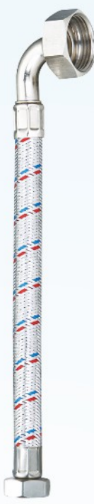
YSF022 不锈钢丝编织管 Stainless Steel Weave Pipe Ø25mm 配置 To configure SUS202/EPDM 规格 Specification F1/2xF3/4(40/60CM)
