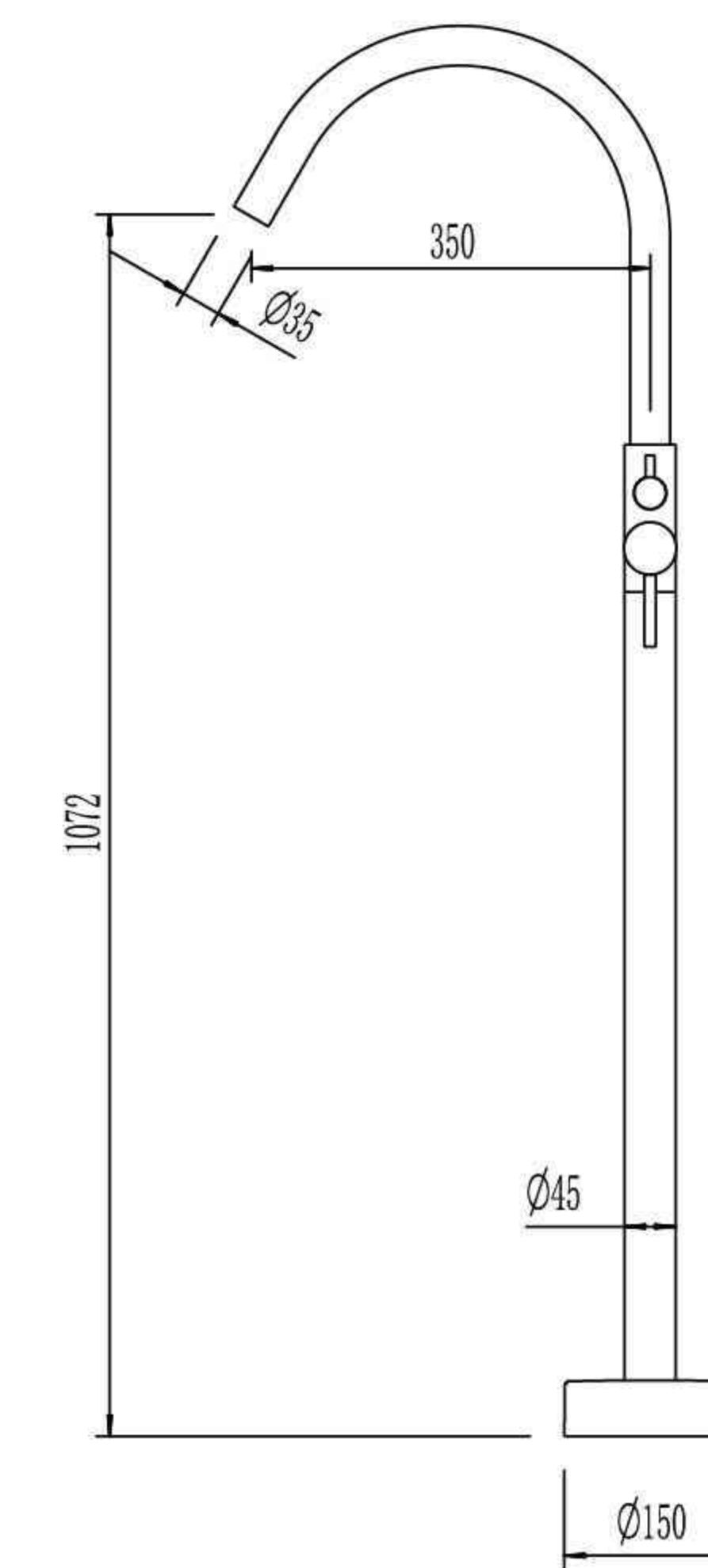
FS2020 Free-standing Bathtub Mixer
