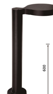
SJ-JCP057 尺寸: \varnothing 260 \times 180 \times 600 LED 12W 铝制品,PC罩
