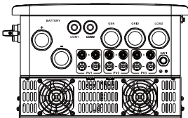
SUN-10/12K-SG05LP2-US-SM3
