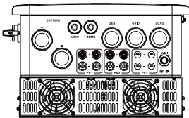
SUN-8K-SG05LP2-US-SM2
