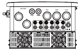
SUN-10/12K-SG05LP2-US-SM3
