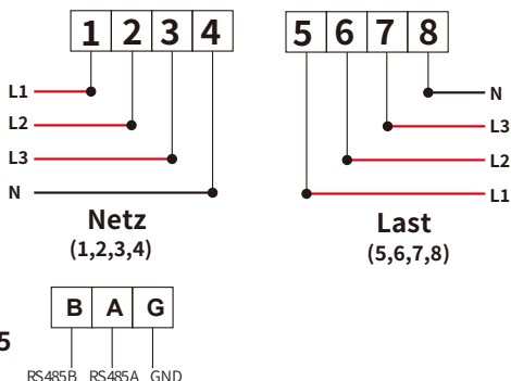
Abb. 7.3 EASTRON-Messer
