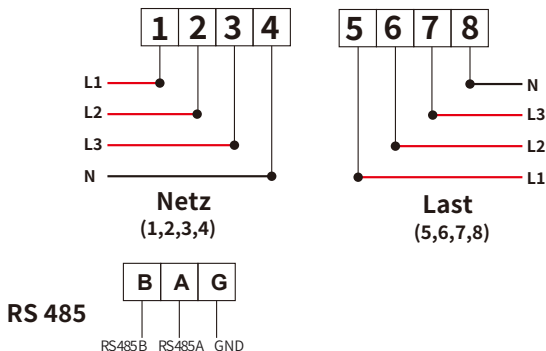
Abb. 7.20 EASTRON-Messer
